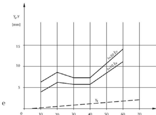
Picture 17. BetonWood® building boards flexion change according to time and load
